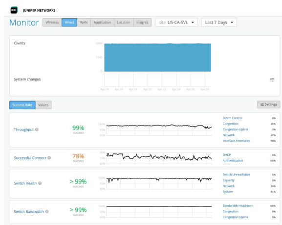
Figure 1: Juniper Mist Wired Assurance service-level expectations screen
